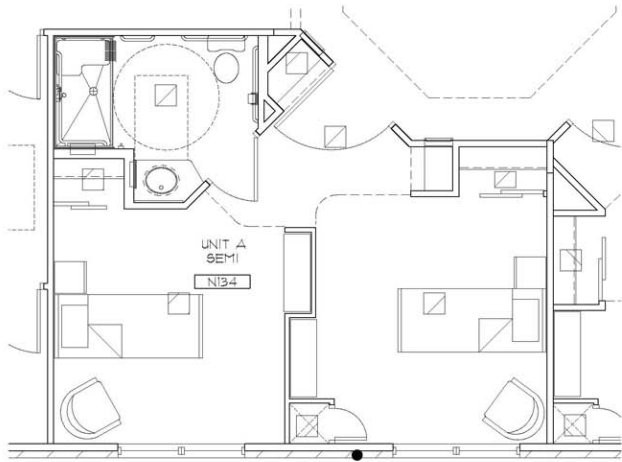
Nursing Unit Type A- Semi-Private \frac{1}{4}''=1'-0'' 407 sf
