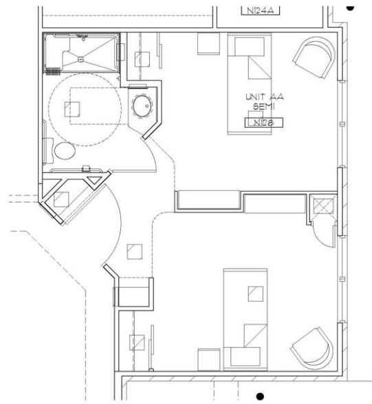
Nursing Unit Type AA- Deep Semi-Private \frac{1}{4}''=1'-0'' 426 sf
